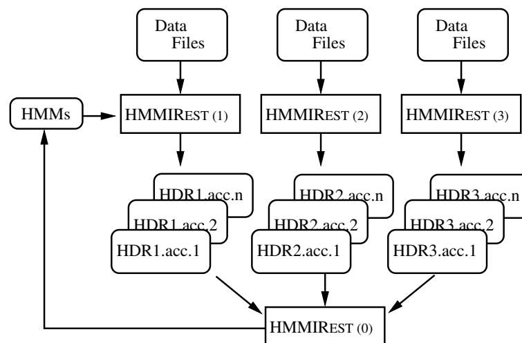
Fig. 8.9 HMMIREst Parallel Operation
