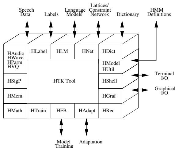
Fig. 2.1 Software Architecture
